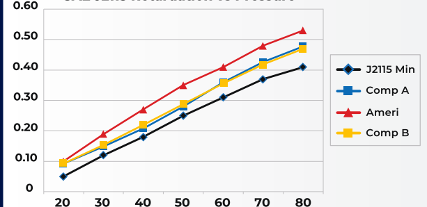
SAE J2115 Retardation vs Pressure
