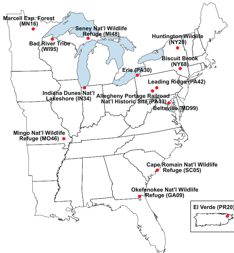
Sites monitoring mercury in leaf litterfall in 2013 as part of a special study initiative.
