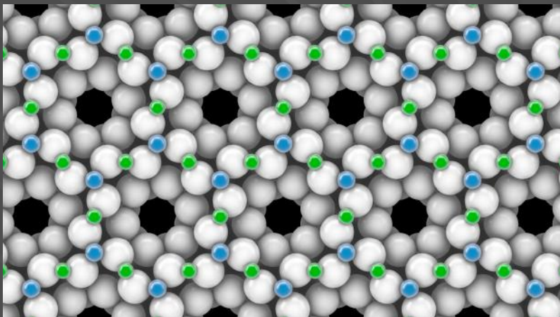
Emerald, \text{Be}_3\text{Al}_2(\text{SiO}_3)_6 green = Be, blue = Al, white = O, Si not visible here Am. Mineral. 71, 977 (1986)
