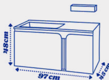
Main Cabinet • 97*45*48
