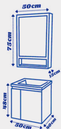
Mirror Box • 50*15*75
