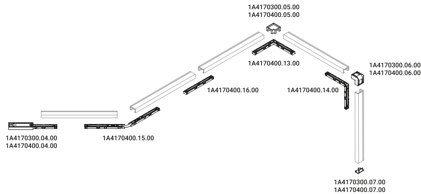
Layout example of wall and ceiling version
