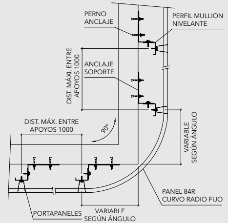
PANEL 84R CURVO
