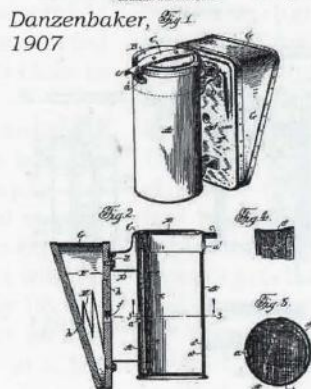
JUNE 4, 1907. T. DANZENBAKER. BEE SMOKER. 856,133
