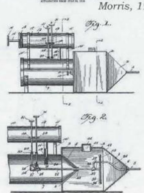
JUNE 23, 1914. L. J. MORRIS. BEE SMOKER. 1,101,466
