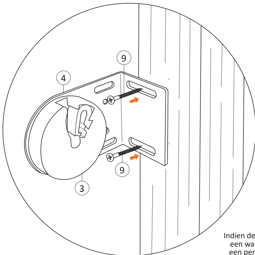
Wandmontage
