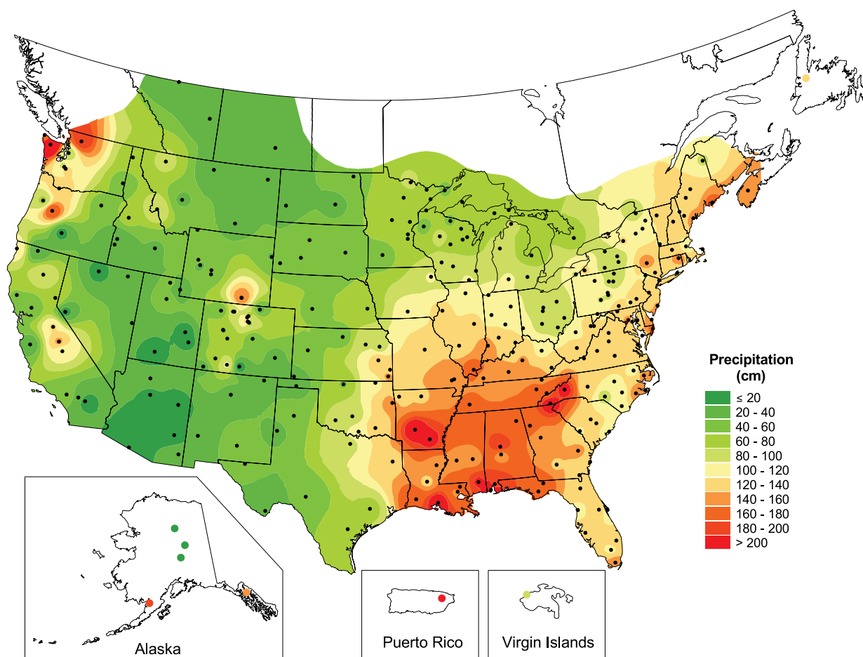
Total precipitation from all NADP wet deposition networks, 2009.
