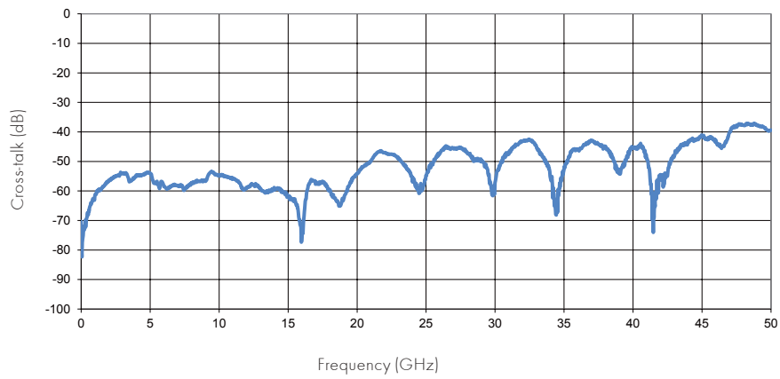
Typical measured cross-talk at PCB transition
