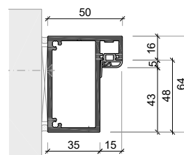
Blockzarge BS48
