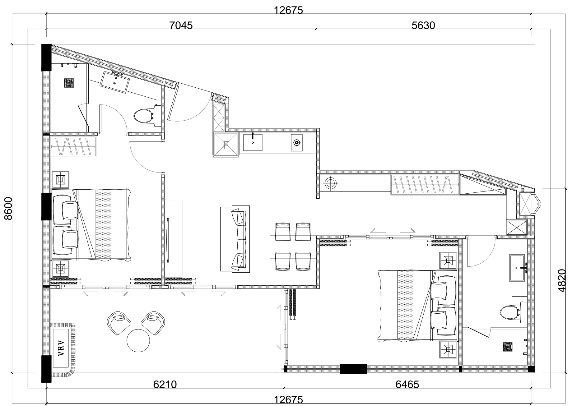
TYPE E AREA 80.85 Sq.m
