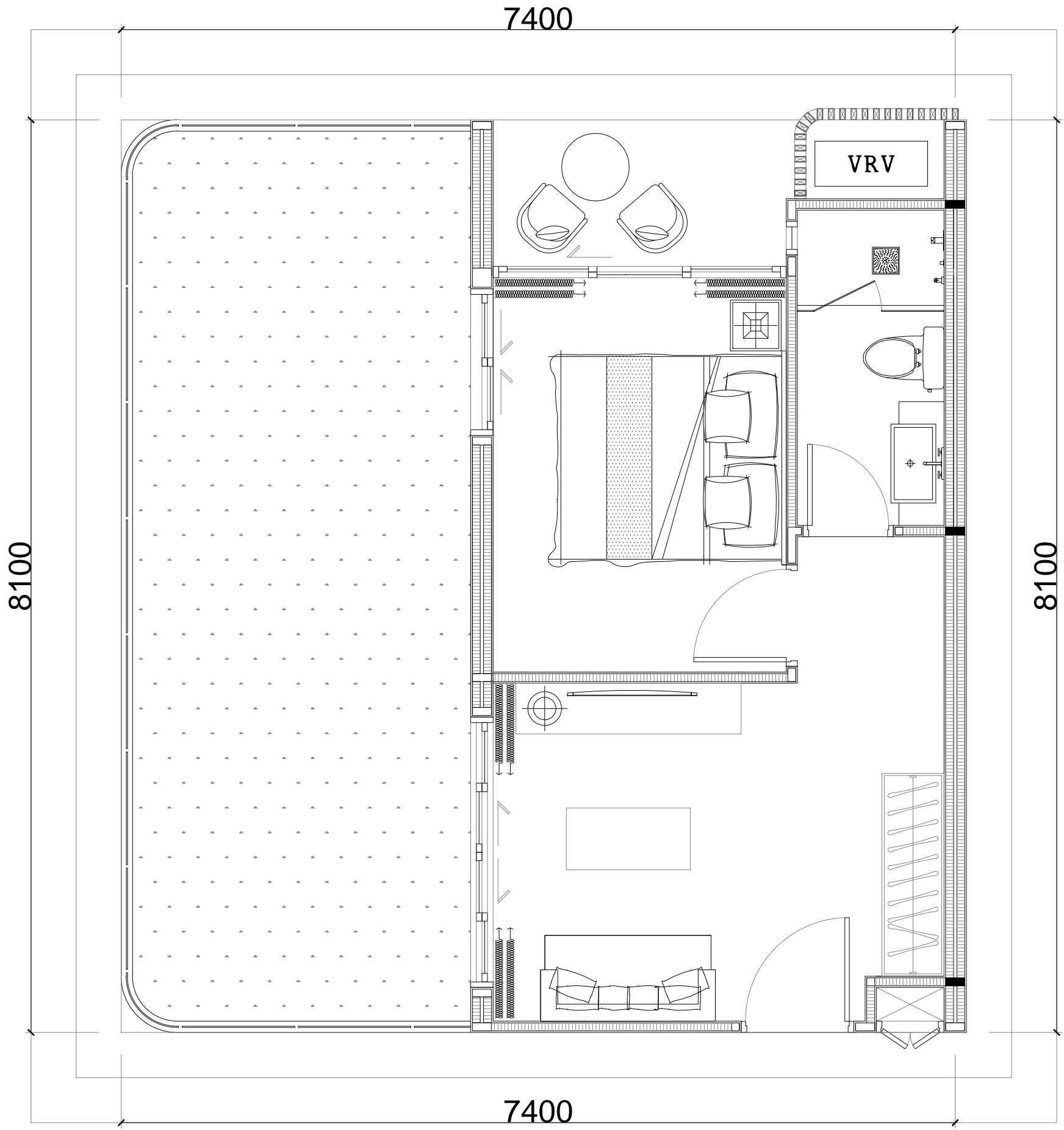
TYPE A4 AREA 57.88 Sq.m
