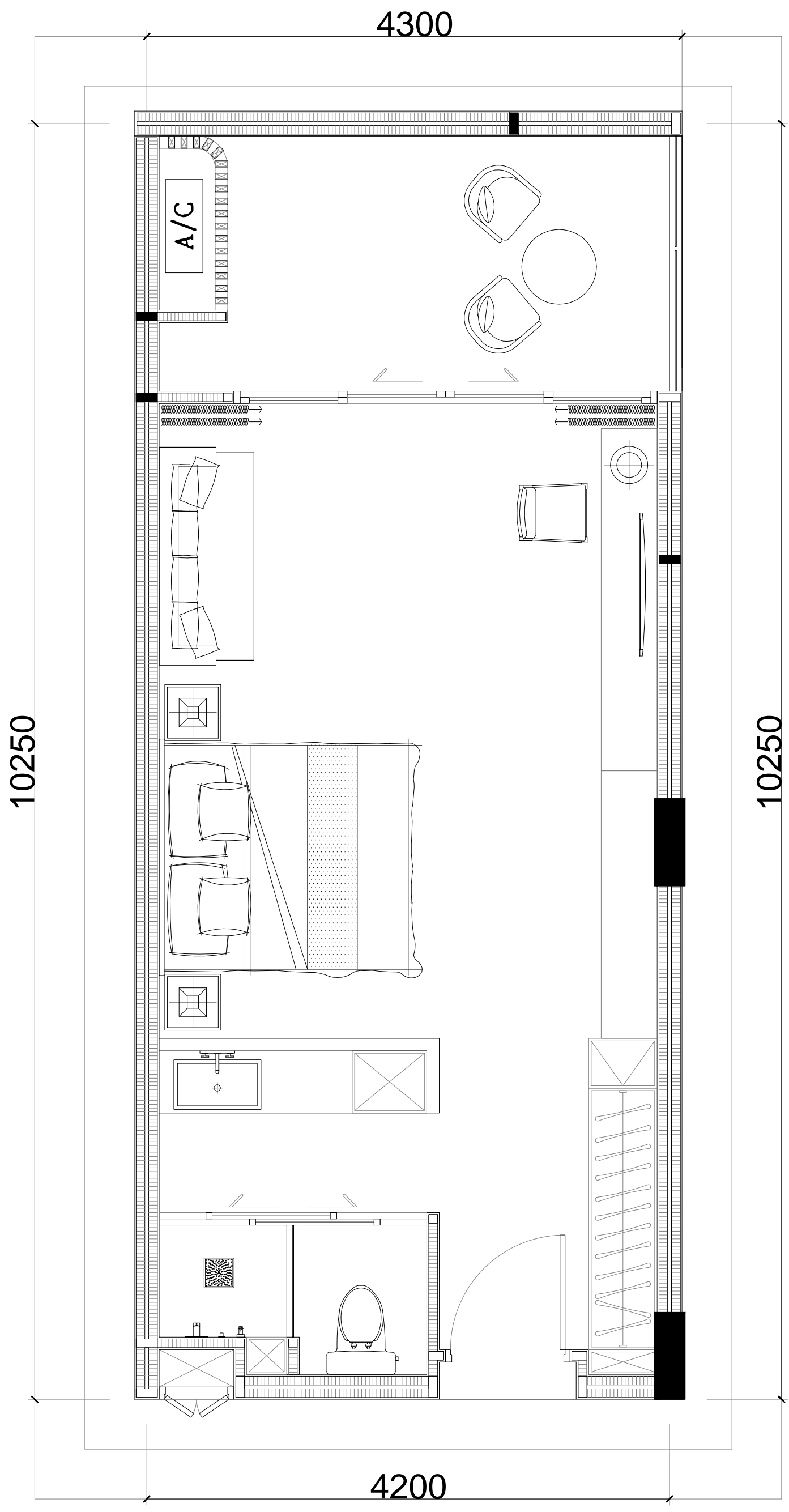
TYPE A9 AREA 41.68 Sq.m
