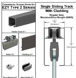
EZY2CLSD Single Sliding Kit with cladding
