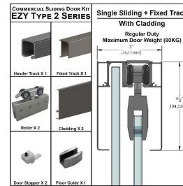
EZY2CLSDP Single Sliding + Fixed Panel Kit with Cladding
