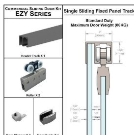
EZYS1SDP Single Door + Fixed Panel Kit
