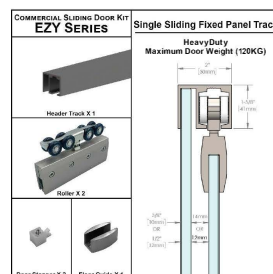
EZYS1HSDP (Heavy Duty) Single Door + Fixed Panel Kit
