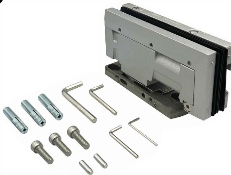
SOL150HONCP Blank Body - Without Cover Plates
