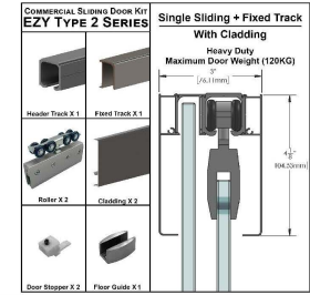
EZY2HDCLSDP (Heavy Duty) Single Sliding + Panel Kit with Cladding
