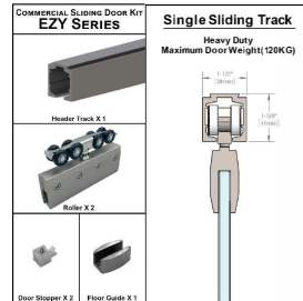
EZYS1HSDS (Heavy Duty) Single Sliding Door Kit
