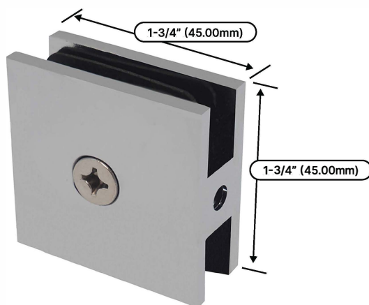
SQU77 Square Hole-in-Glass Style Wall Mount Clamp
