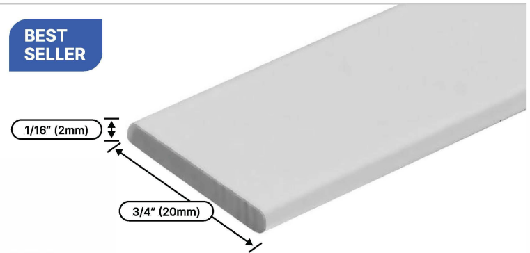
FB144 3/4" Flat Bar For Grid Showers - 144" Length 3/4" Wide X 1/16" Thick
