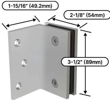
WMB90 Square Wall Mount Bracket - 90°
