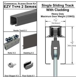
EZY2HDCLSD (Heavy Duty) Single Sliding Kit with Cladding
