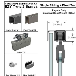
EZY2SDP Single Sliding + Fixed Panel Kit
