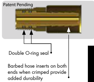
Cross section of LIFESwivel® fitting
