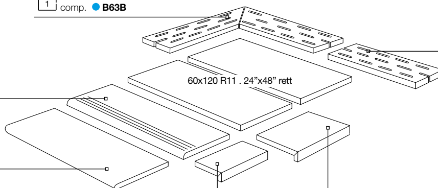
Gradone Costa Retta R11 35x60x5 . 13 3/4" x24"x2" rett
