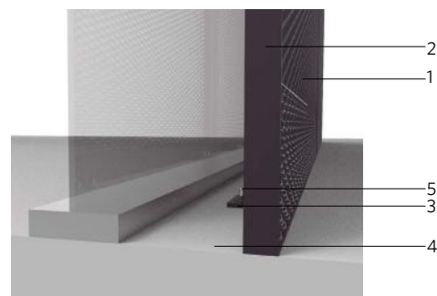
REMATE INFERIOR
