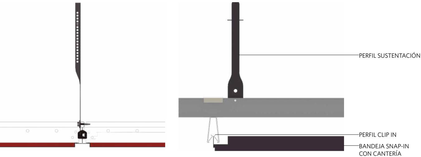
DETALLE CIELO TILE LAY-IN
