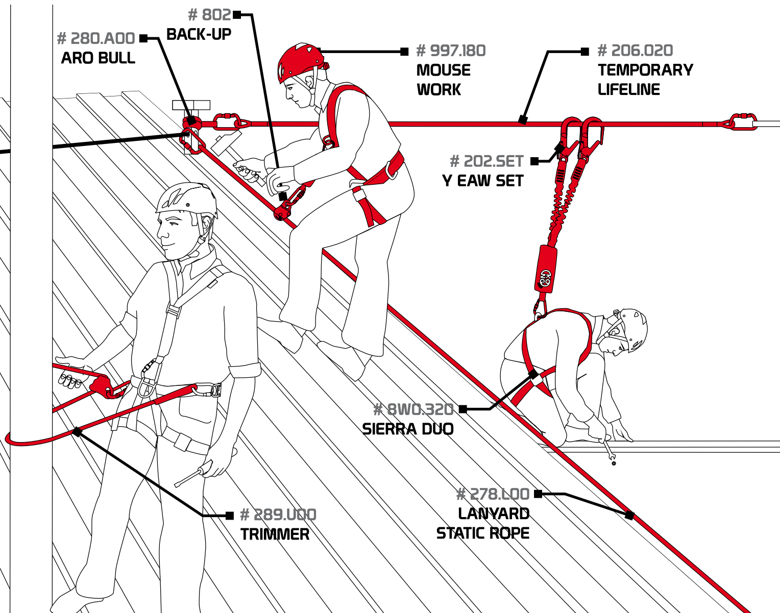
SIERRA DUO ANSI
