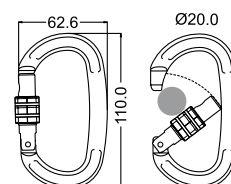
STAINLESS STEEL auto block twist lock
