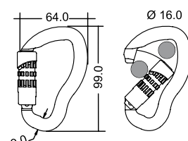
ALU ALLOY auto block twist lock
