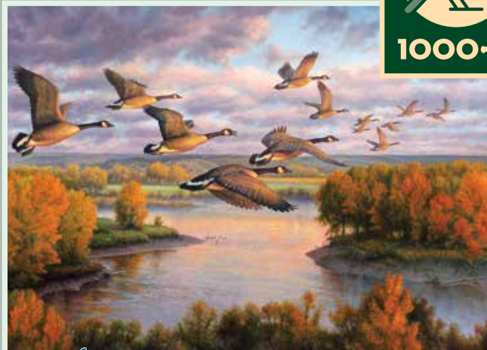
40280 | Migration
