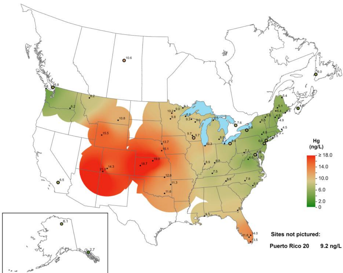
Total mercury concentration, 2024.
