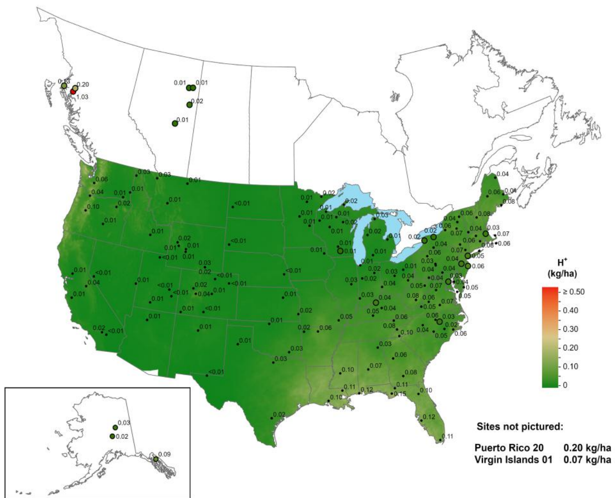
Hydrogen ion wet deposition, 2024.
