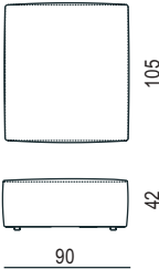
POUF OTTOMAN 90 X 105
