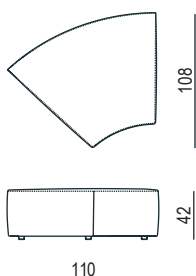
POUF SEMICURVO SEMI ROUND OTTOMAN 110 X 108
