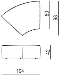
POUF SEMICURVO SEMI ROUND OTTOMAN 104 X 98
