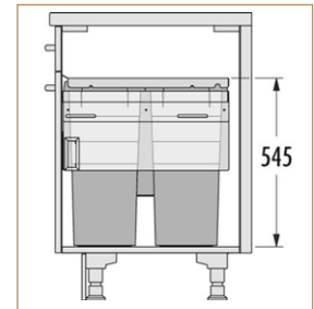
Waste Management can be integrated into base cabinets
