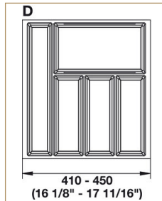
Cutlery Tray, for 21" and 21 11/16" Deep Drawer, Plastic
