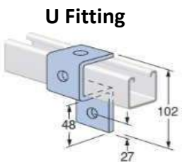
U Fitting
