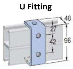
U Fitting
