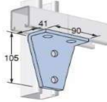
45 Degree Plate Angle
