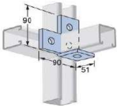
LH Angle Plate
