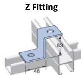
Z Fitting
