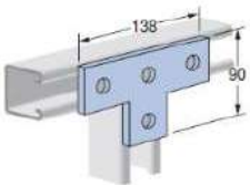
T Flat Plate Fitting
