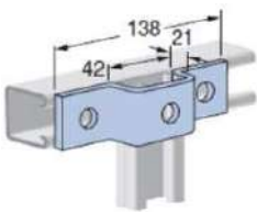
Beam Clamp
