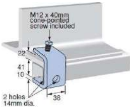
Beam Clamp
