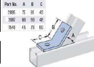
L Plated Braced
