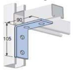
L Plate Angle Fitting
