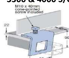
Beam Clamp
