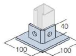
Base Plates
