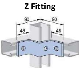
Z Fitting
