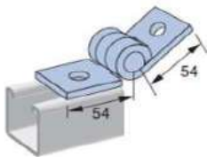
External Channel Hanger
