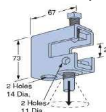
Beam Clamp
