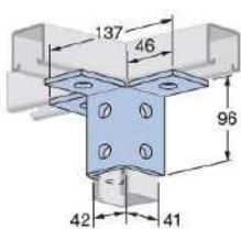
Wing Fitting
