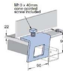
Beam Clamp 1000 & 2000 S/C
