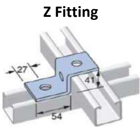
Z Fitting
