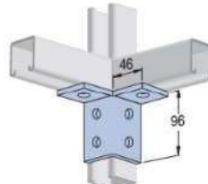
Wing Fitting
