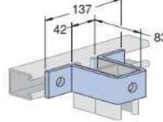
U Fitting
