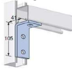
Angle Fitting 90 Degrees
