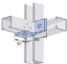
Flat Angle Plate
