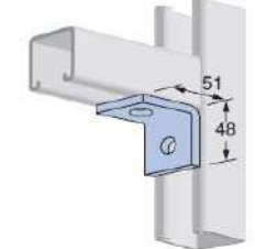
Angle Plate
