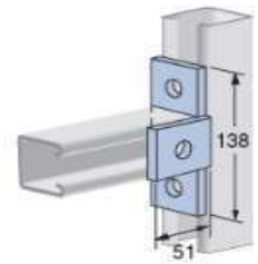
Angle Fitting 90 Degrees
