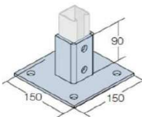
Base Plates
