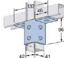
Wing Fitting
