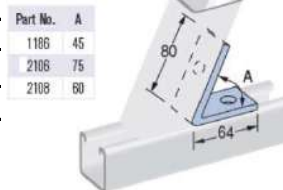
45 Degree Angle Plate
