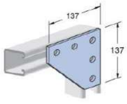
Flate Plate Fitting
