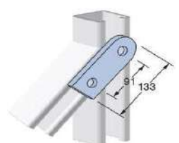
Flat Angle Plate
