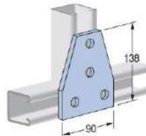
Flate Plate Fitting
