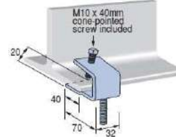
Beam Clamp
