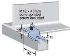
Beam Clamp
