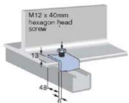
Beam Clamp
