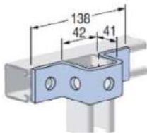
U Fitting
