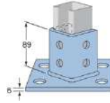
Double Base Plate
