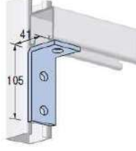
Angle Fitting 90 Degrees
