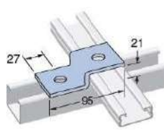
Z Fitting
