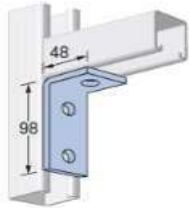
Channel Fitting Single Pivot Arm
