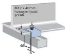
Beam Clamp
