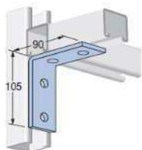
L Plate Angle Fitting
