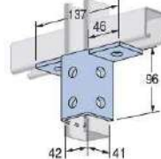
Wing Fitting
