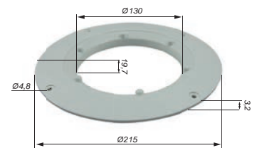
Ceiling Light Ring Dachlampering Aro de Empotrar para Plafones 6901316/2569001/2569005
