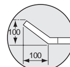
Detail 2 - Top view Detalle 2 - Vista superior
