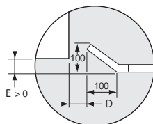
Detail 1 - Top view Detalle 1 - Vista superior
