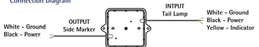
Connection Diagram
