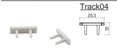
Endcap
