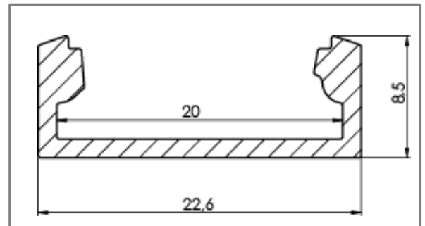
Dimensioni – Dimension H8 x L22mm
