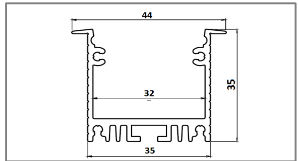
Dimensioni – Dimension H35 x L44mm
