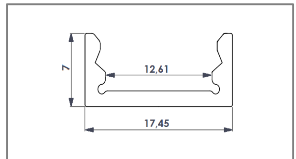
Dimensioni – Dimension H7 x L17mm
