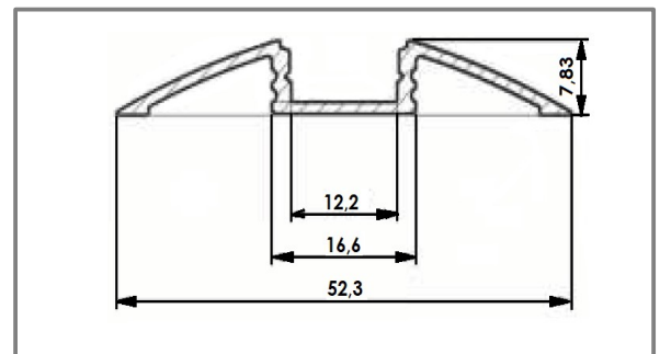
Dimensioni – Dimension H9 x L55mm
