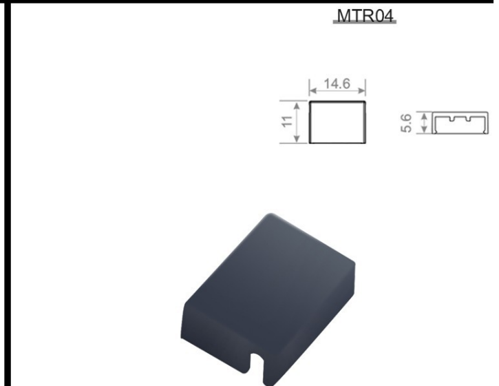
Track Connector
