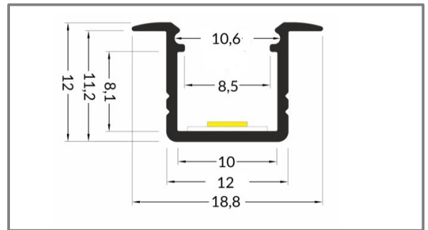
Dimensioni – Dimension H12 x L18,8mm
