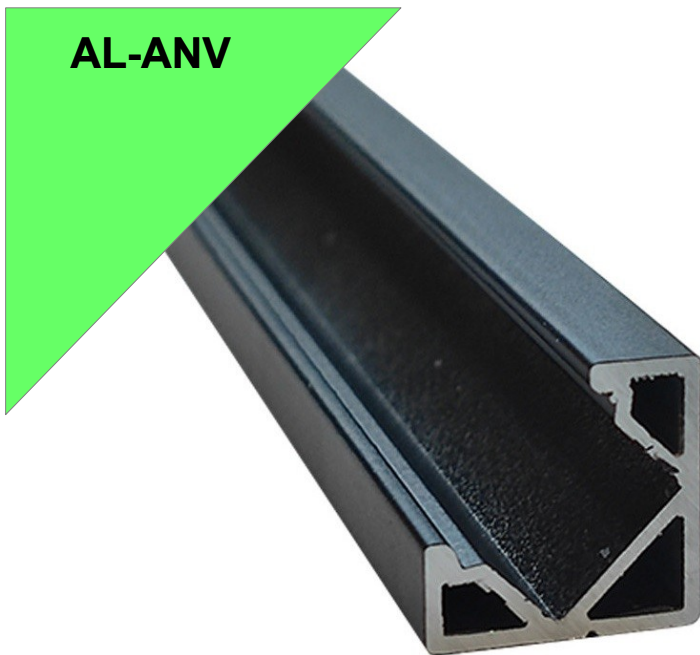
Dimensioni – Dimension H19 x L19mm
