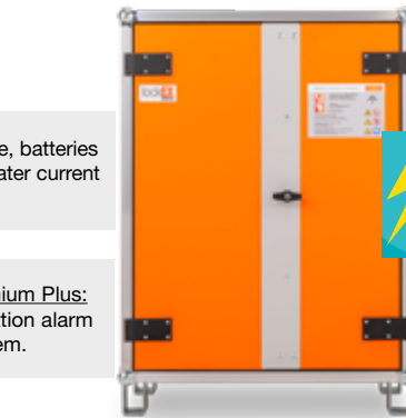
Battery charging cabinet 8/10 Premium Plus 3-phase
