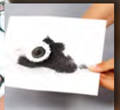
MAGNETIC FIELDS
