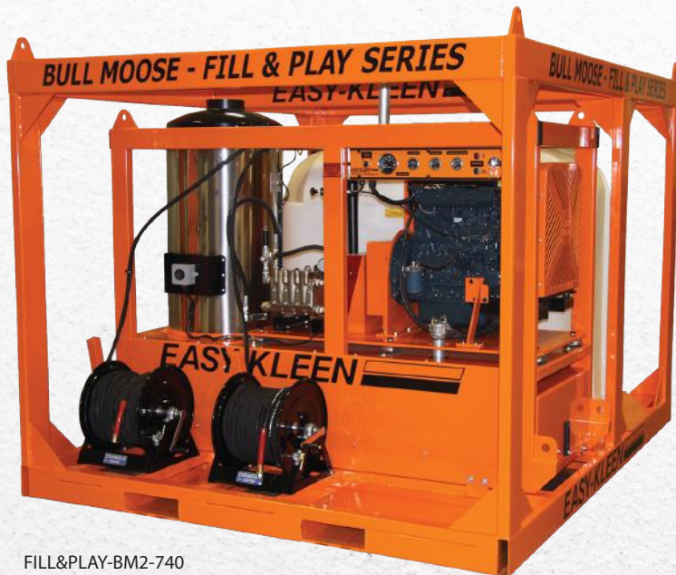
FILL&PLAY-BM2-740 Frame Option, pg. 71
