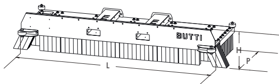
QUOTE SEDI FORCHE INTERNE INTERNAL FORK SEATS DIMENSIONS
