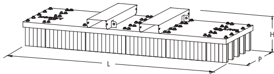
QUOTE SEDI FORCHE INTERNE INTERNAL FORK SEATS DIMENSIONS
