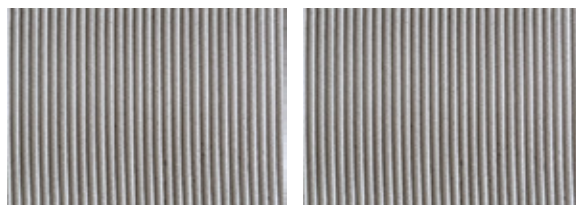
OK Spreading on substrate and tile in same direction
