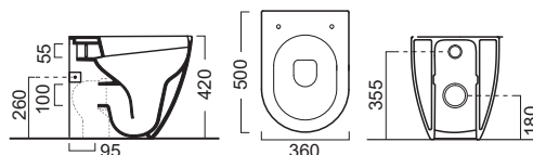
MS86SC SUPER Slim Soft Close
