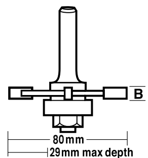
TX CUTTER
