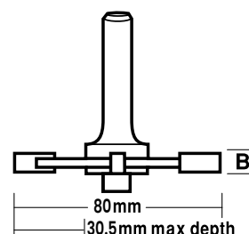
TX CUTTER
