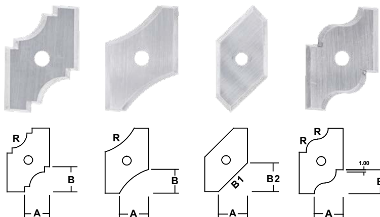
RMST 301
