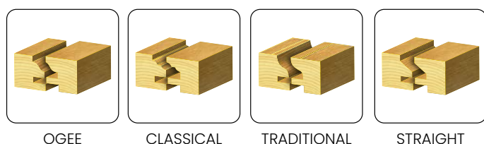
OGEE
