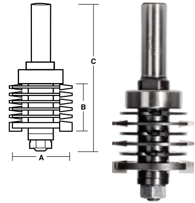
4 Cutters
