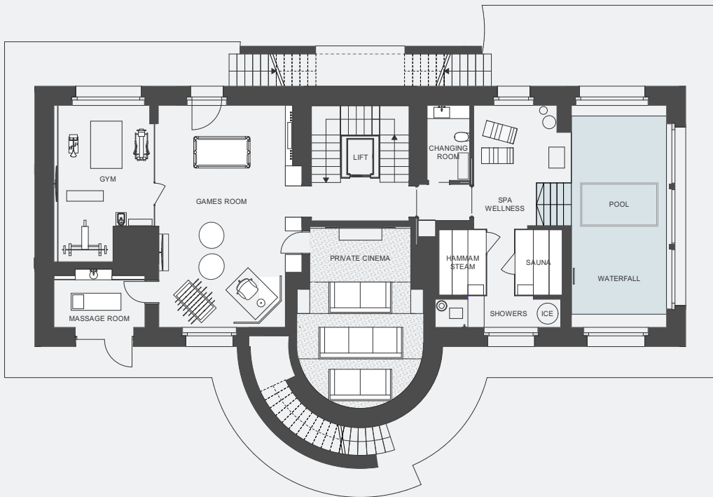
GROUND FLOOR
