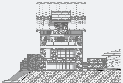
WEST ELEVATION
