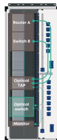
Monitoring via external TAP and OOO switch
