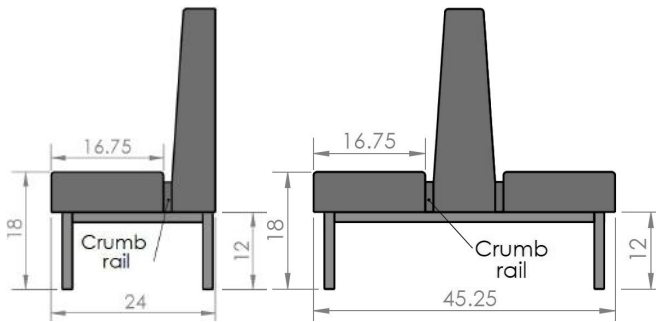
Pacific Booth Dimensions - 42" std. height
