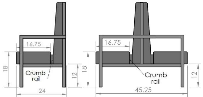
Reef Booth Dimensions - 38" std. height
