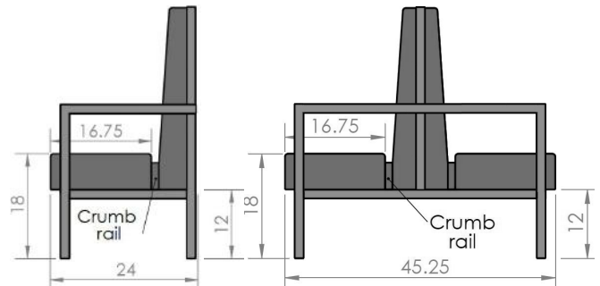
Reef Booth Dimensions - 38" std. height
