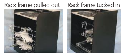
Rack frame pulled out
