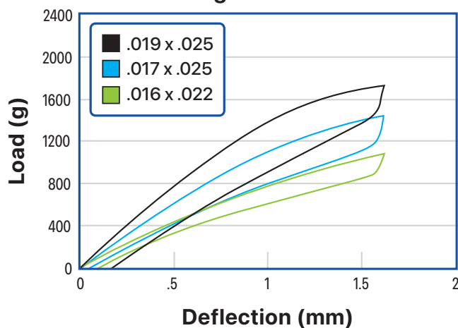
Rectangular Force Chart
