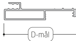
Aluminiumforing tre/aluminiumvindu
