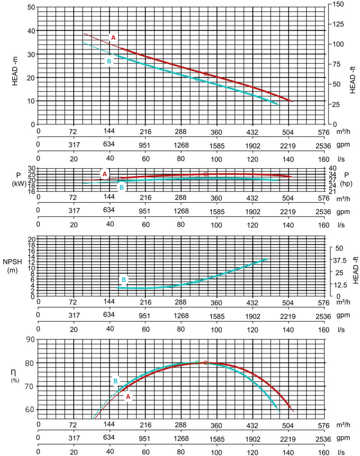
Curves at Speeds: A 1900 rpm B 1800 rpm
