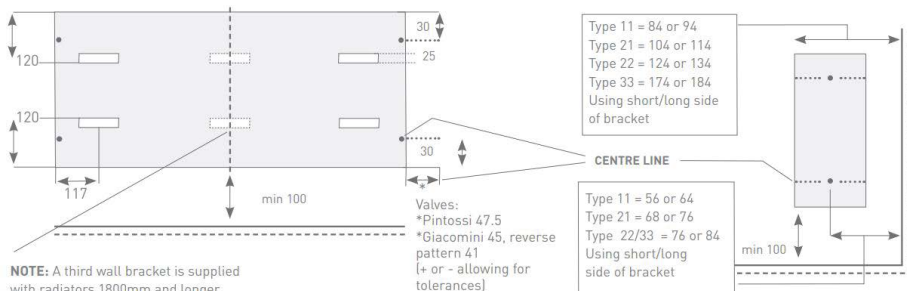
Standard bracket supplied with DeLonghi radiators
