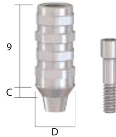
Temporary Abutment [Non-Hex]
