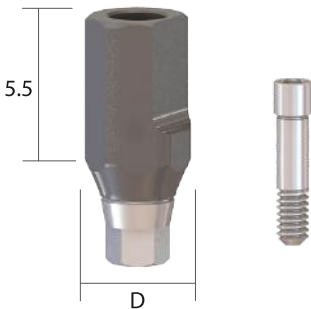
Scan Body Diameter Collar Code Ø4.5 1.5mm SSB25M
