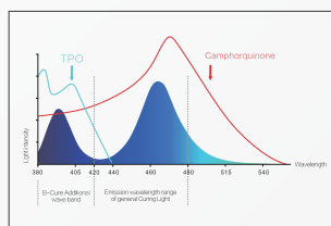
O-light plus spectral curve & resin spectral absorptivity
