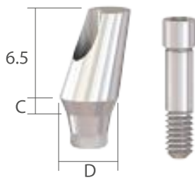
20° Angled Abutment [Hex]
