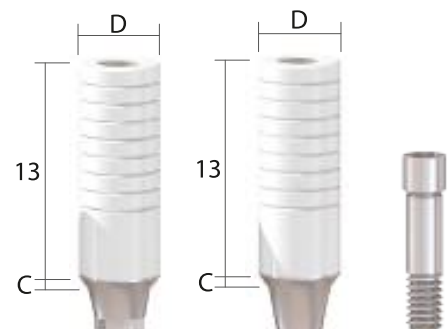
Cr-Co UCLA Abutment [Hex] / [Non-Hex]
