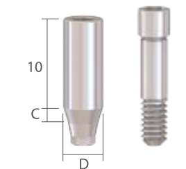
Cementation Abutment [Non-Hex]
