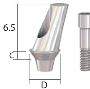
20° Angled Abutment [Non-Hex]
