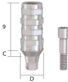
Temporary Abutment [Hex]
