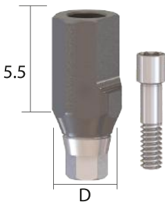
Scan Body Diameter Collar Code Ø4.0 1.5mm SSB21M
