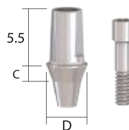
Cementation Abutment [Non-Hex]
