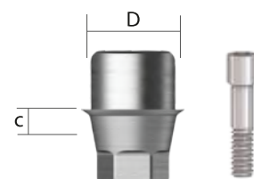
LINK Abutment [Hex]
