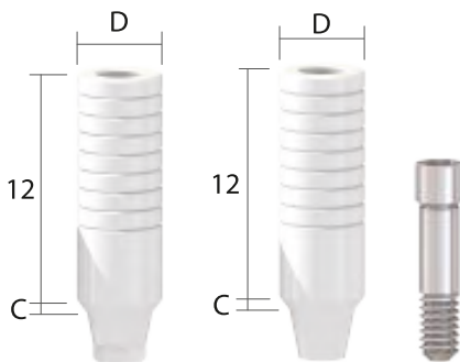
UCLA Abutment [Hex] / [Non-Hex]
