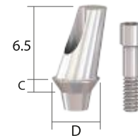
15° Angled Abutment [Non-Hex]
