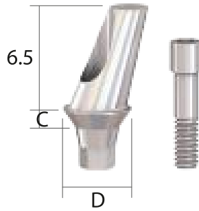
20° Angled Abutment [Hex]
