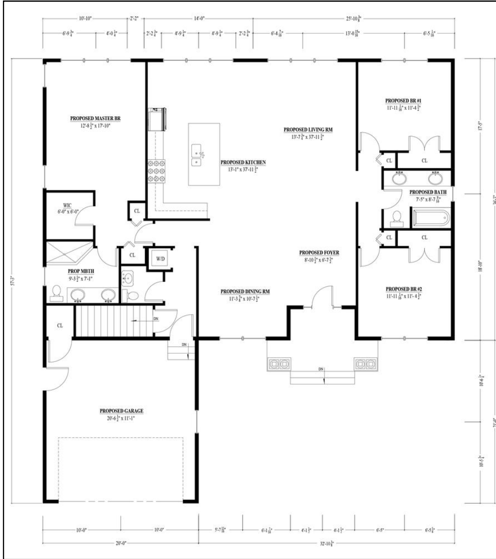
Floor Plan Option 1: Total Floor Area: 1,850 sq ft
