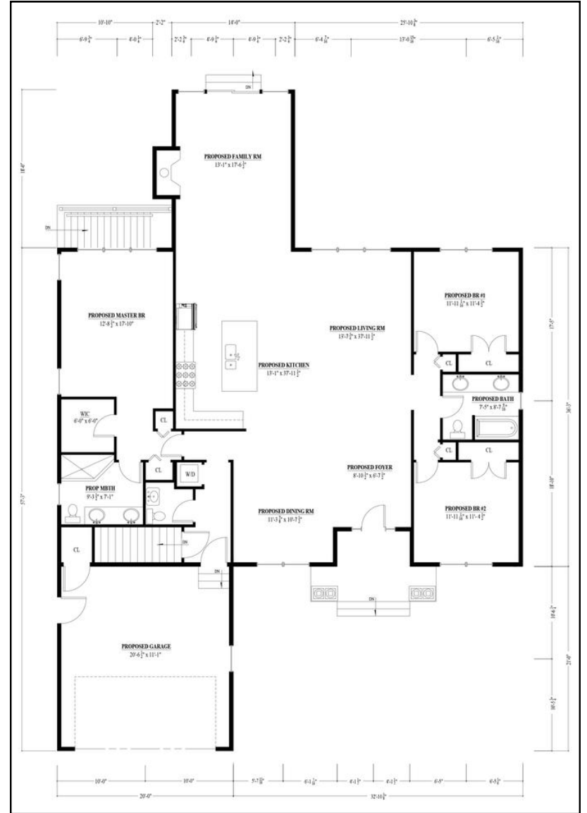
Floor Plan Option 2: Total Floor Area: 2,024 sq ft
