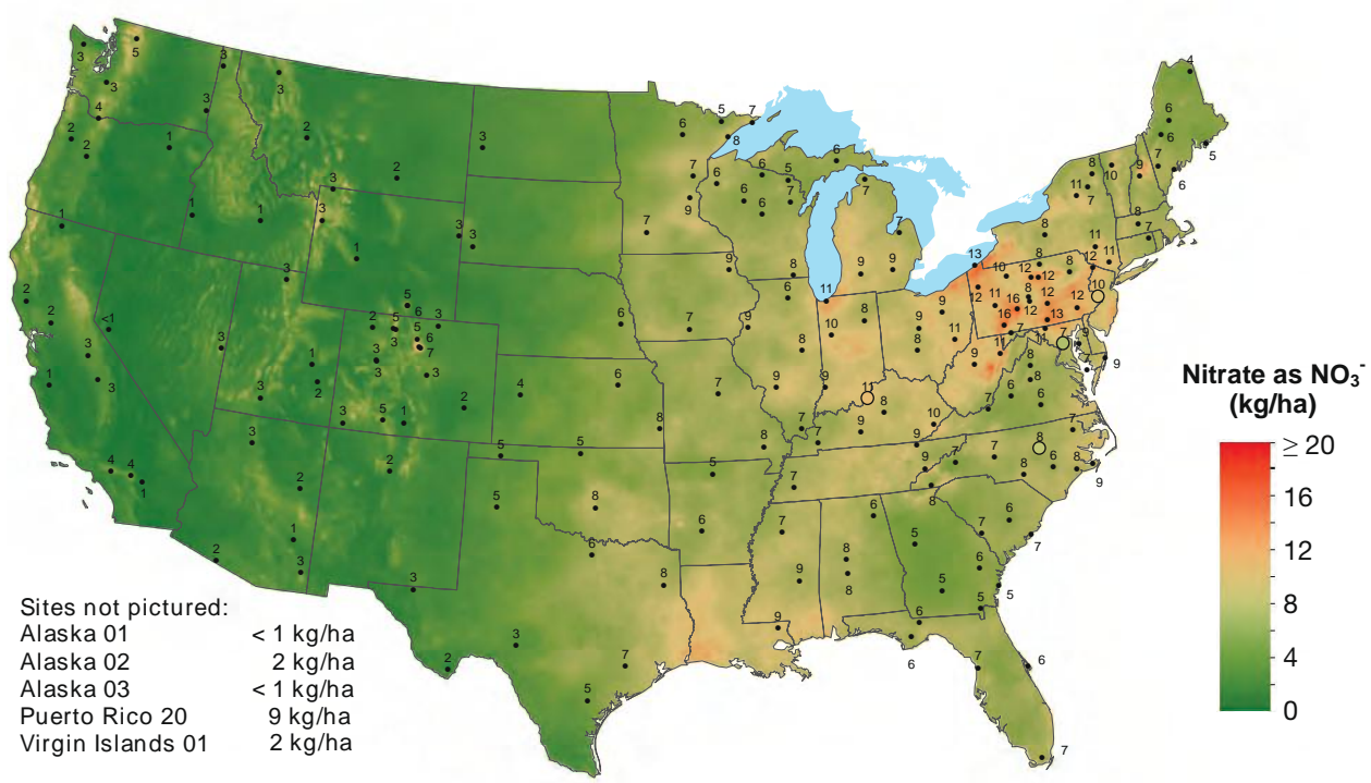
Nitrate ion concentration (top) and wet deposition (bottom), 2012.
