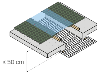
SINGLE NET distance from the walking surface \leq 50 cm
