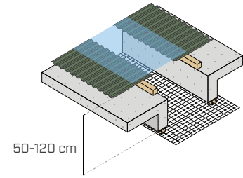
SINGLE NET distance from the walking surface 50–120 cm
