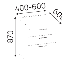
DRAWER BASE
