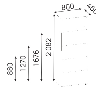
MODEX OPEN
