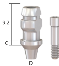
Impression Coping [Pick-up] Close Tray Non-Hex
