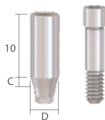
Milling Abutment [Hex]
