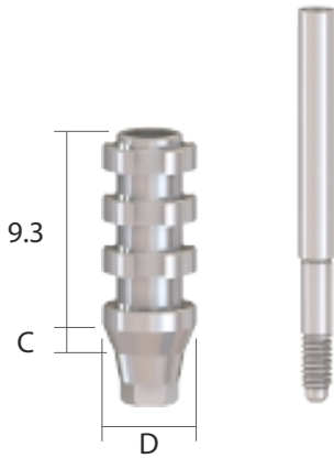
Impression Coping [Pick-up] Open Tray Hex
