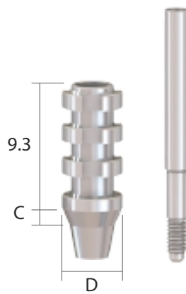
Impression Coping [Pick-up] Open Tray Non-Hex
