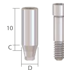
Cementation Abutment [Non-Hex]
