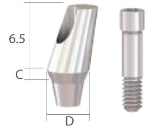
15° Angled Abutment [Hex]
