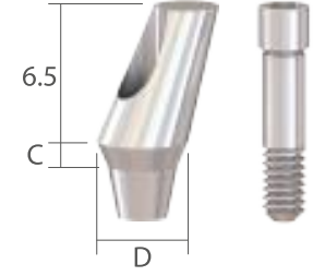
20° Angled Abutment [Non-Hex]
