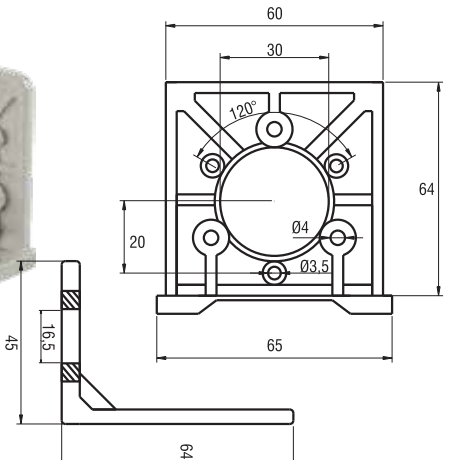
SF50B Square flange
