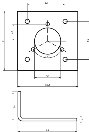
SF58B Square flange
