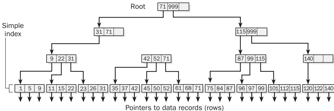
B-tree. A B-tree index structure.
